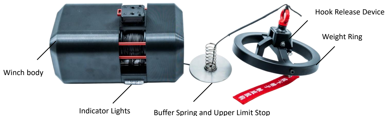
FIG 3-2-1 Diagram 1 of the 15KG UAV payload winch
