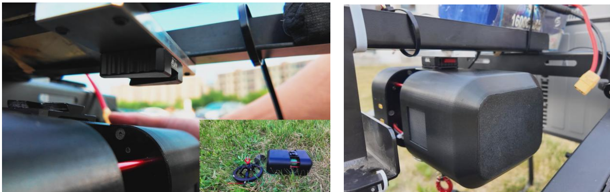
FIG 5-2-1 The installation of the winch body on the aircraft platform
