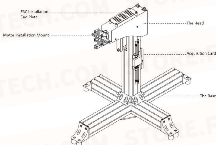
FIG 4-1-1 Thrust stand structure
