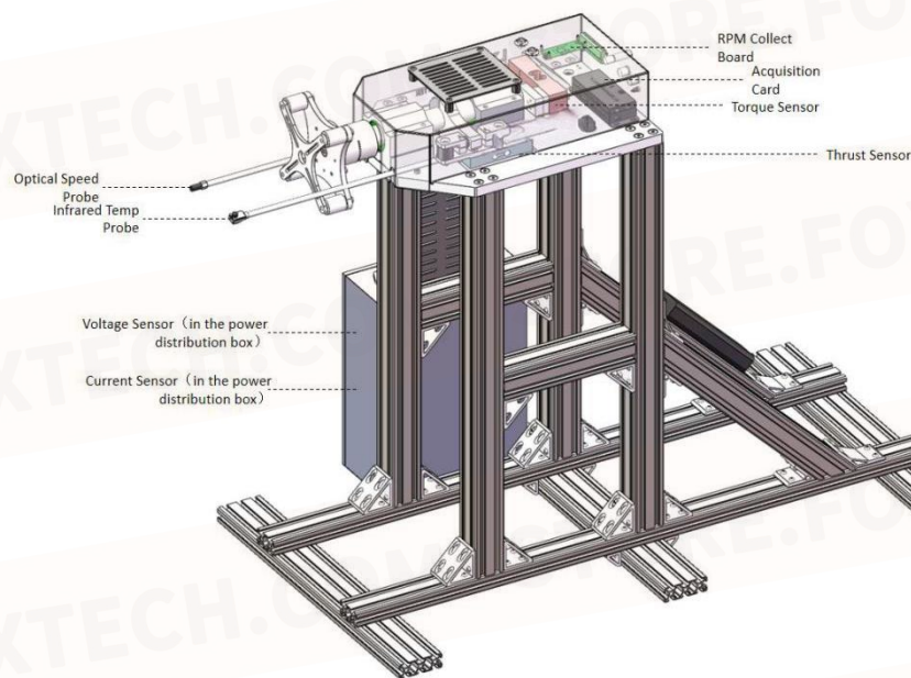
FIG 4-2-2 Sensor Position
