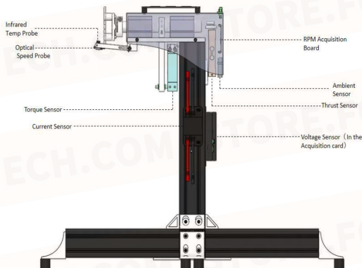
FIG 4-1-2 Sensor Position
