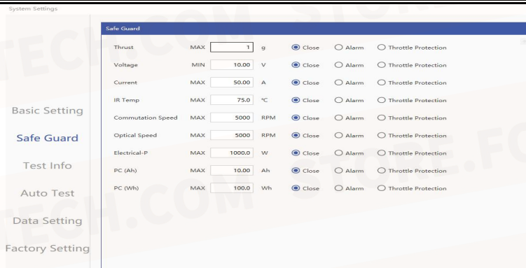
FIG 5-1-3 Safe Guard Interface
