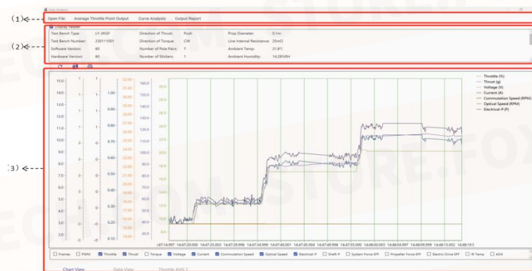
FIG 6-1 Data Analysis Interface
