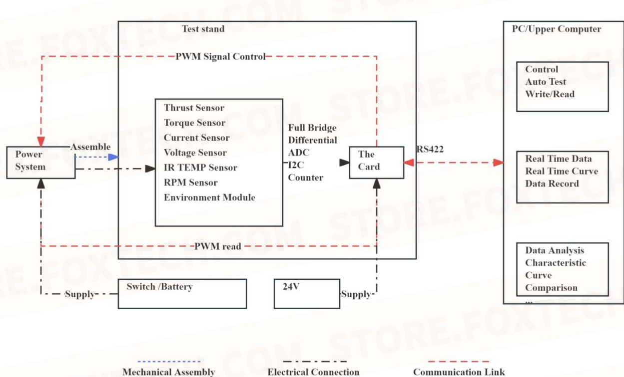
FIG 3-3-1 The system operation logic diagram
