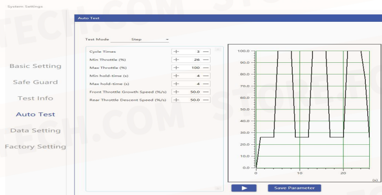
FIG 5-1-10 Auto Test-Step Mode
