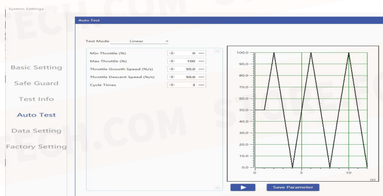
FIG 5-1-9 Auto Test-Linear Mode
