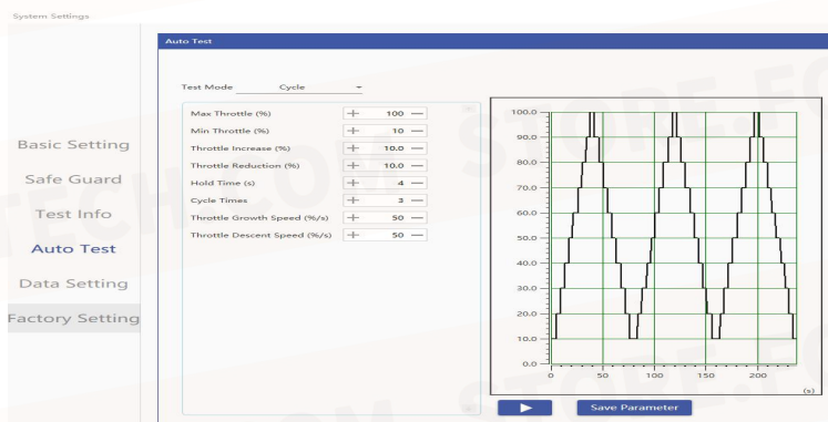
FIG 5-1-6 Auto Test-Cycle Mode
