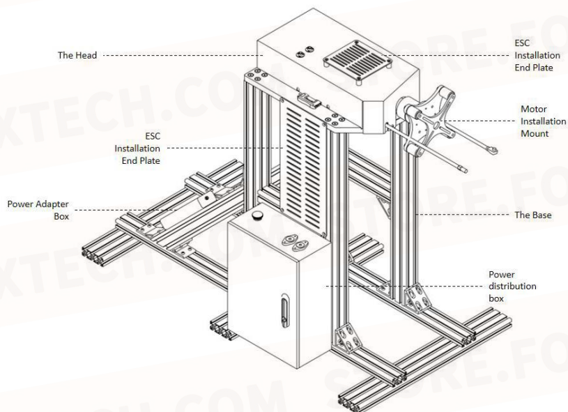
FIG 4-2-1 Thrust stand structure
